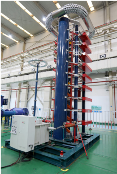
— Lightning Impulse Test Device
