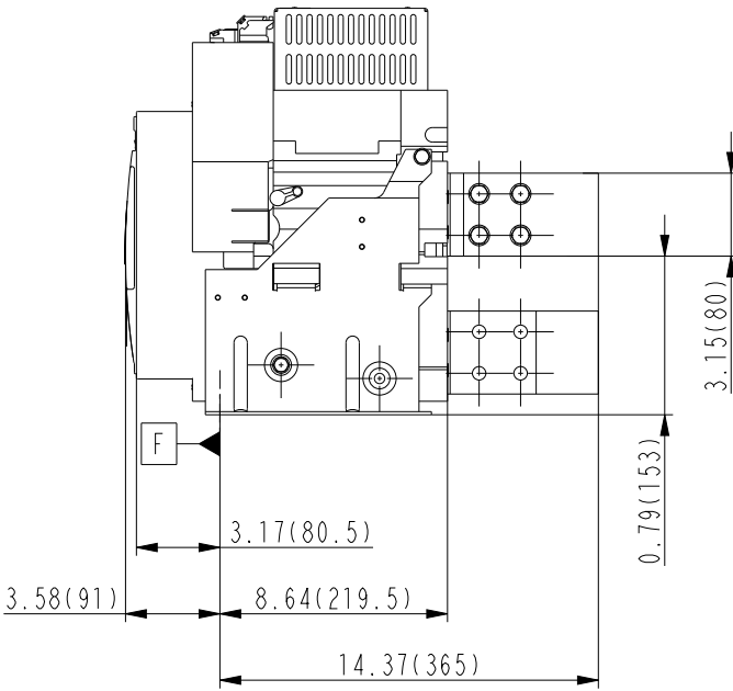
2500A_Type D_Vertical_Reverse
