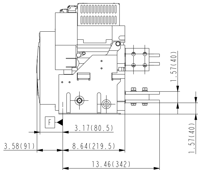
800_2000A_Type D_Verical
