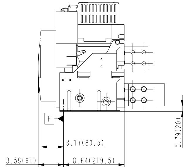
2500A_Type C_Vertical
