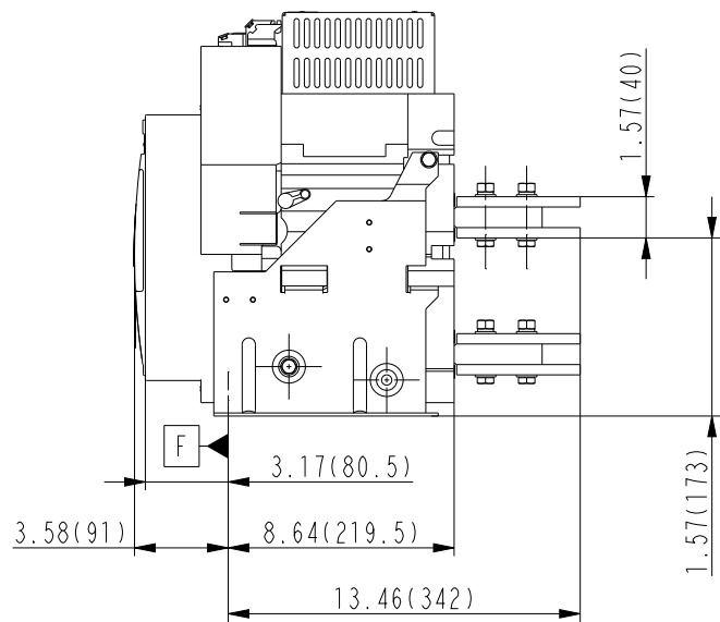
800_2000A_Type D_Horizontal_Reverse
