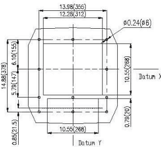
panel perforating size
