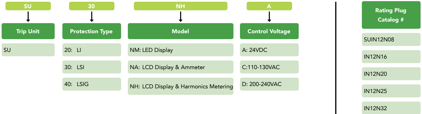
A32/A40 Trip Unit Models Display Options
