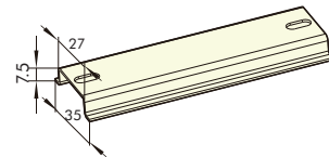
Mounting dimension of externally mounted handle
