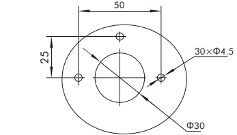
Mounting dimension of externally mounted handle
