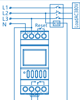
Figure 5 Wiring diagram of 3-phase control (contactor coil AC380V)
