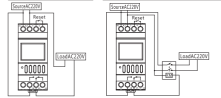
Figure 2 Wiring method of single phase control Figure 3 Wiring method of single phase expanded capacity control (contactor coil AC220V)
