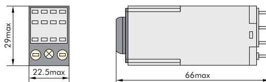
JSZ6 overall and mounting dimension
