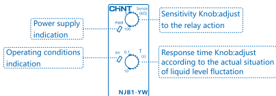
Figure 5 Panel Diagram
