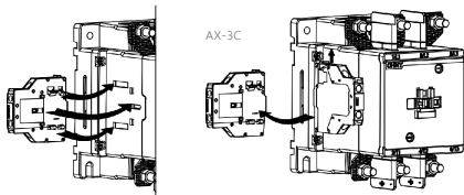
Figure 3-3 Installation of AX-3C
