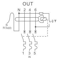
Figure 4 Wiring diagram
