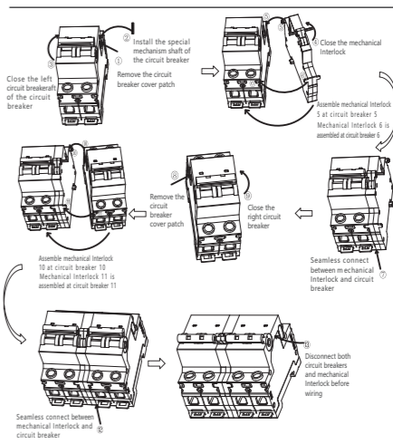
Figure 6 LMI-B1 / XB mechanical interlock assembly mode diagram
