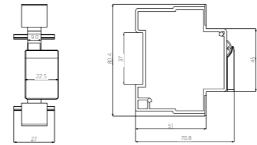
Figure 1 LMI-12 mechanical interlock appearance and installation dimension
