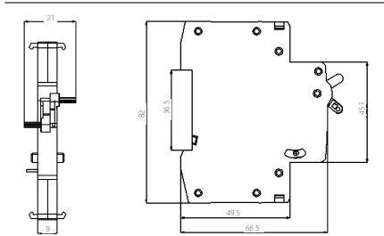
Figure 3 LMI-B1 mechanical interlock appearance and installation dimension
