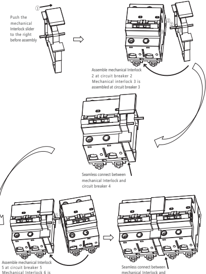
Figure 5 LMI-12 / 13 mechanical interlock assembly mode diagram
