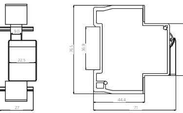
Figure 2 LMI-13 mechanical interlock appearance and installation dimension
