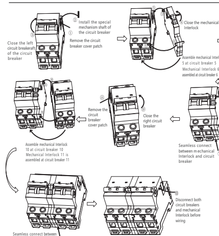
Figure 6 LMI-B1 / XB mechanical interlock assembly mode diagram
