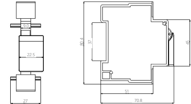
Figure 1 LMI-12 mechanical interlock appearance and installation dimension
