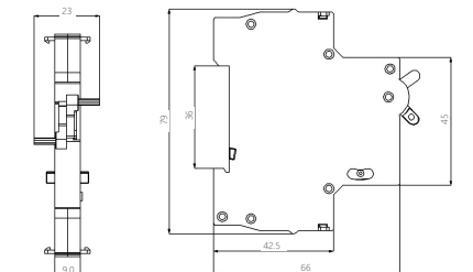
Figure 4 LMI-XB mechanical interlock appearance and installation dimension
